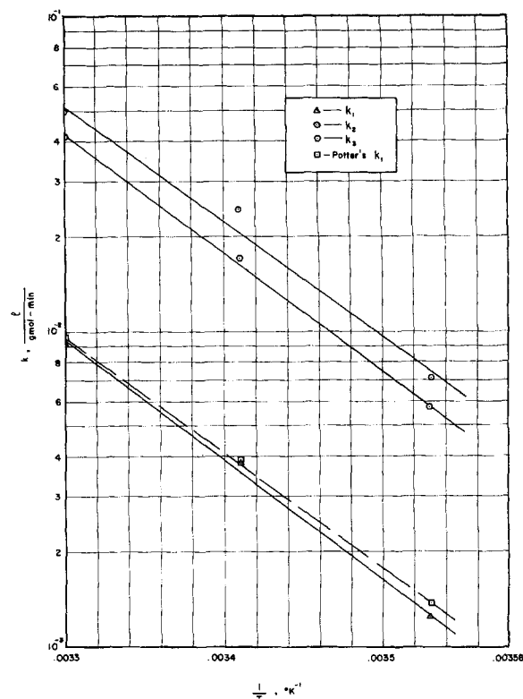
Fig. 4. Arrhenius plot for ethanolamine synthesis.
